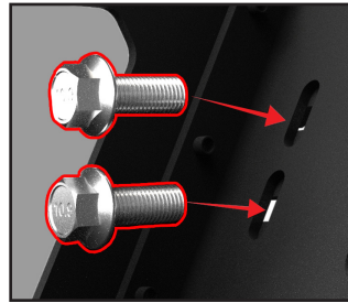
Fig. 16-Inside Basket View
